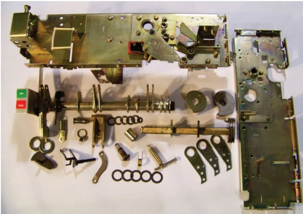
Typical 5 kV mechanism components
